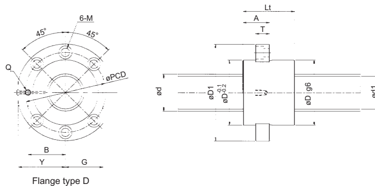
Flange type D
